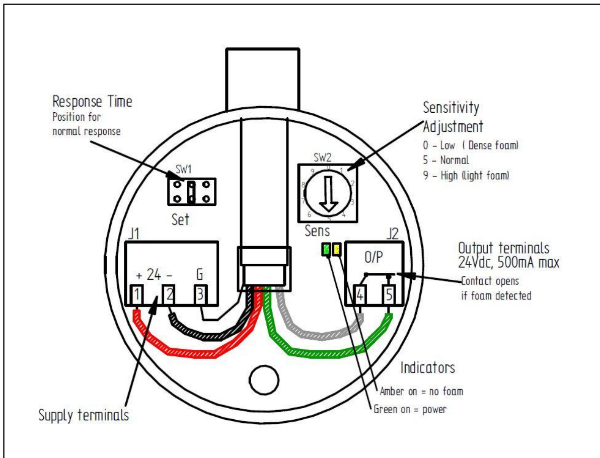
Figure 1 – CONNECTIONS and ADJUSTMENTS
